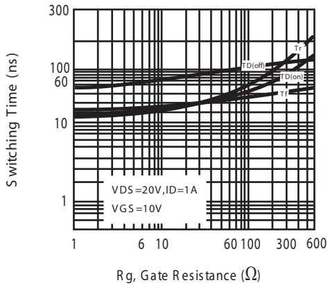
Figure 12. switching characteristics
