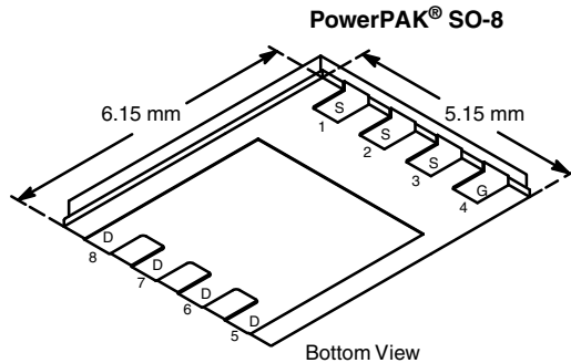
Ordering Information: SiR870DP-T1-GE3 (Lead (Pb)-free and Halogen-free)
