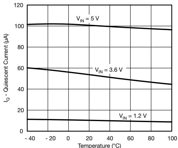
Fig. 5 - Quiescent Current vs. Temperature
