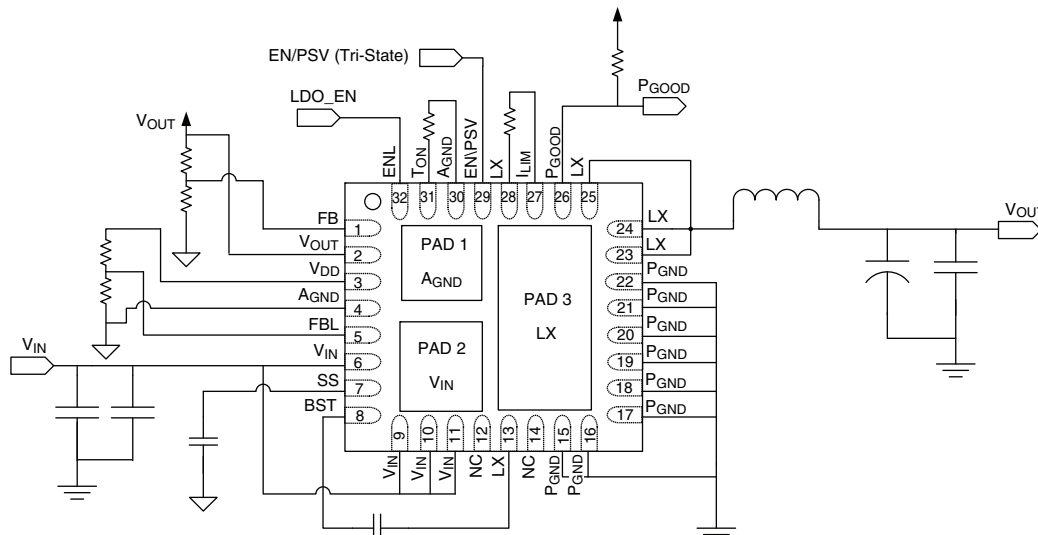
Typical Application Circuit for SiC401A/B (PowerPAK MLP55-32L)
