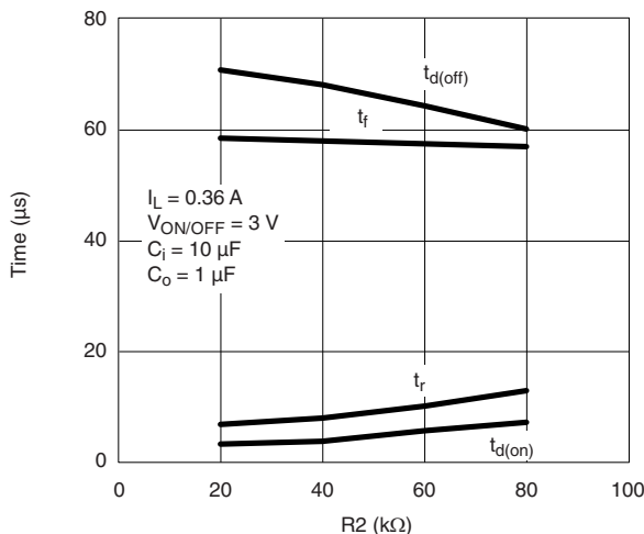
Switching Variation R2 at V_{IN} = 4.5 \text{ V} , R1 = 300 \text{ kW}
