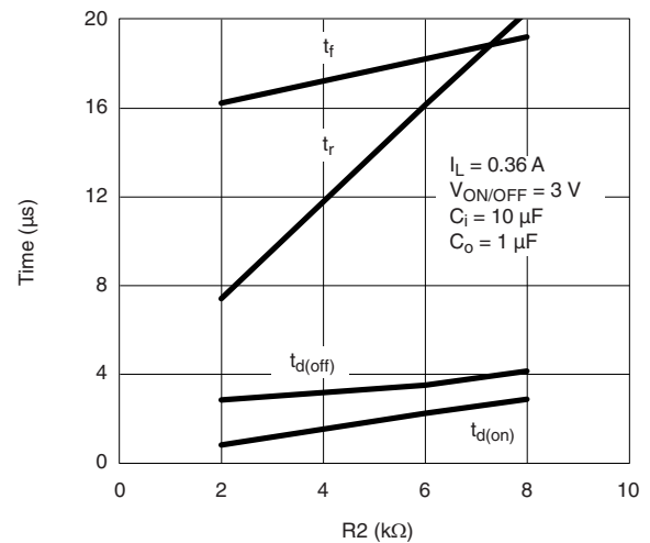
Switching Variation R2 at V_{IN} = 1.8 \text{ V} , R1 = 20 \text{ kW}
