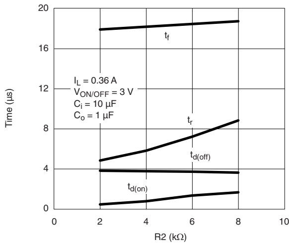
Switching Variation R2 at V_{IN} = 2.5 \text{ V} , R1 = 20 \text{ kW}
