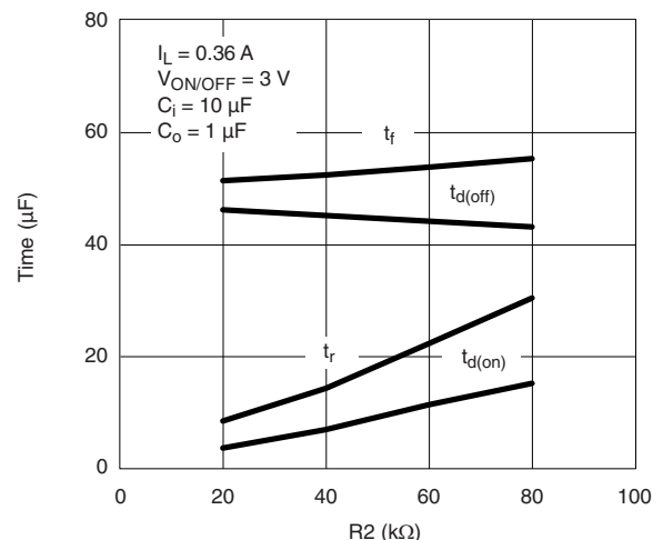
Switching Variation R2 at V_{IN} = 2.5 \text{ V} , R1 = 300 \text{ kW}
