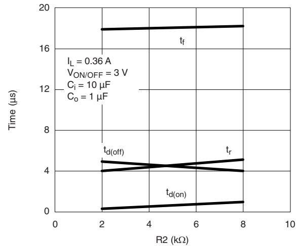
Switching Variation R2 at V_{IN} = 4.5 \text{ V} , R1 = 20 \text{ kW}
