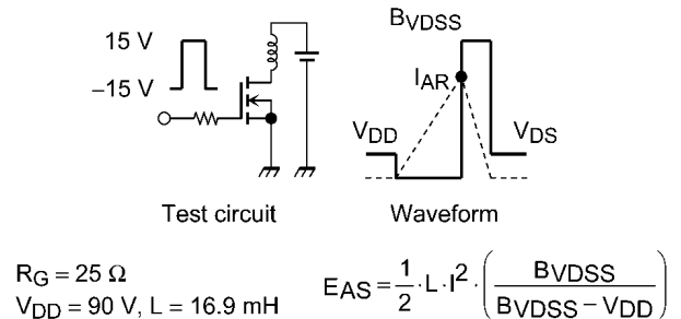
Fig. 8.16 Test Circuit/Waveform
