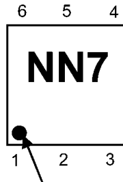
Polarity marking Fig. 6.1 Marking
