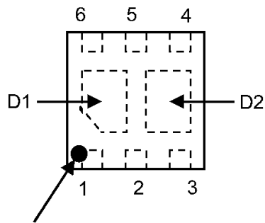
Polarity marking (on the top) *Electrodes : on the bottom Fig. 6.2 Pin Condition(Top View)
