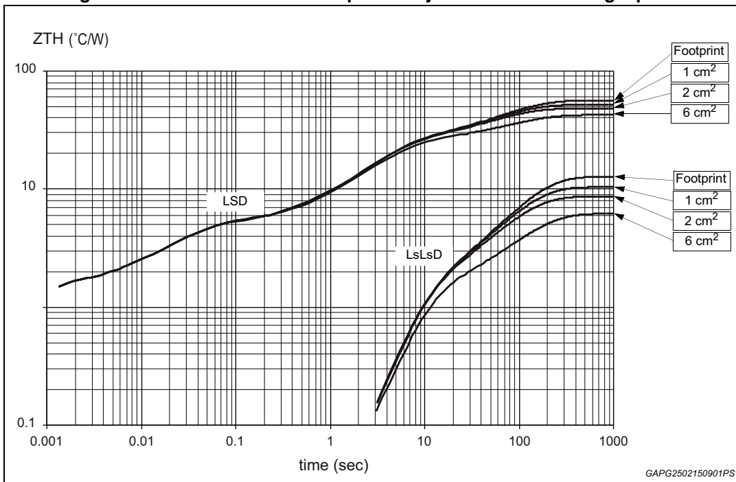
Figure 41. SO-28 LSD thermal impedance junction ambient single pulse
