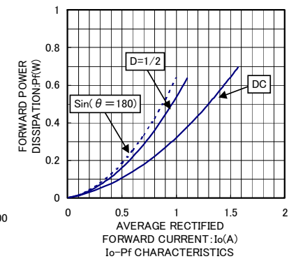
Io-Pf CHARACTERISTICS
