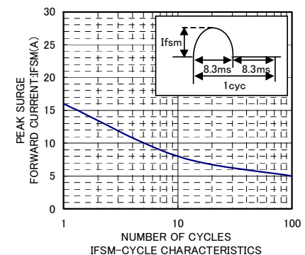
IFSM-CYCLE CHARACTERISTICS
