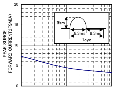
IFSM-CYCLE CHARACTERISTICS
