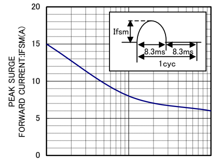
IFSM-CYCLE CHARACTERISTICS
