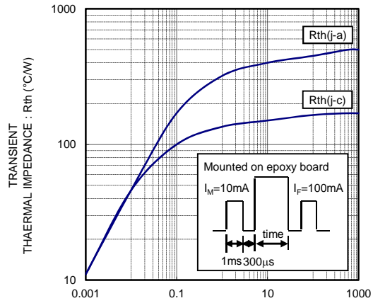
Rth-t CHARACTERISTICS
