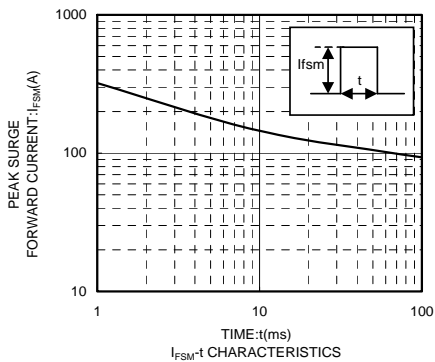
I_{FSM}-t CHARACTERISTICS
