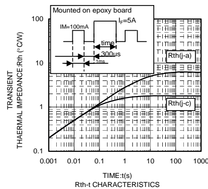
R_{th}-t CHARACTERISTICS
