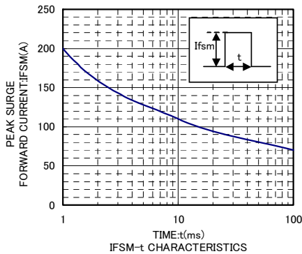
IFSM-t CHARACTERISTICS
