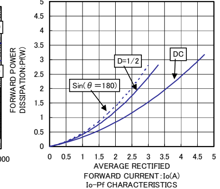
I0-Pf CHARACTERISTICS
