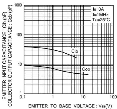
Fig.7 Collector output capacitance vs. collector-base voltage Emmitter input capacitance vs. emmitter-base voltage
