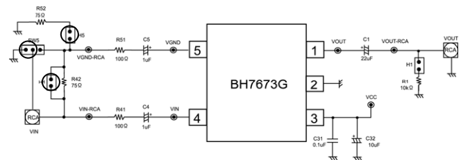
Fig.6 CMRR measurement
