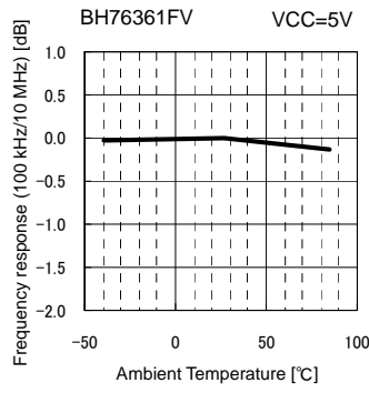
Fig.38 G_F vs. Ambient Temperature
