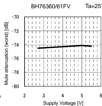
Fig.43 MT(worst) vs. Supply Voltage
