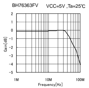
Fig.80 Frequency Response
