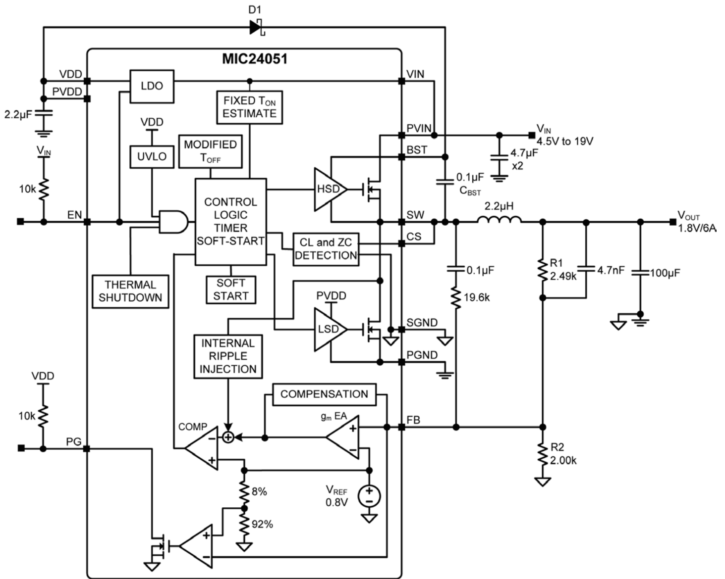
Figure 1. MIC24051 Block Diagram
