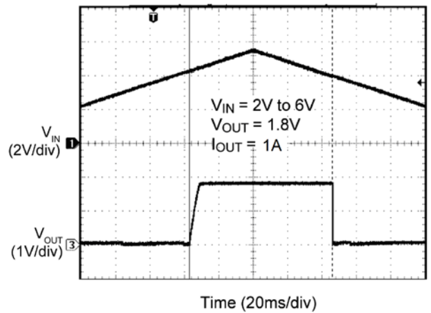
V_{IN} UVLO Threshold
