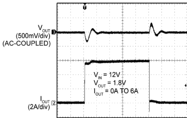
Transient Response
