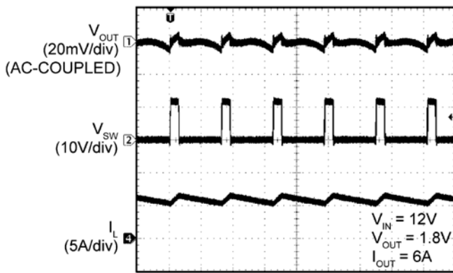
Switching Waveforms
