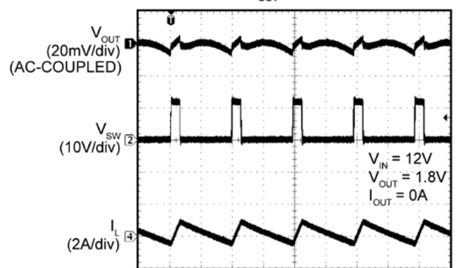
Switching Waveforms
