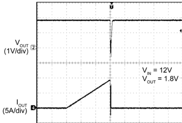
Output Current-Limit Threshold
