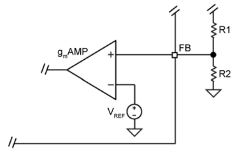
Figure 8. Voltage-Divider Configuration
