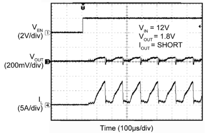
Enable into Short
