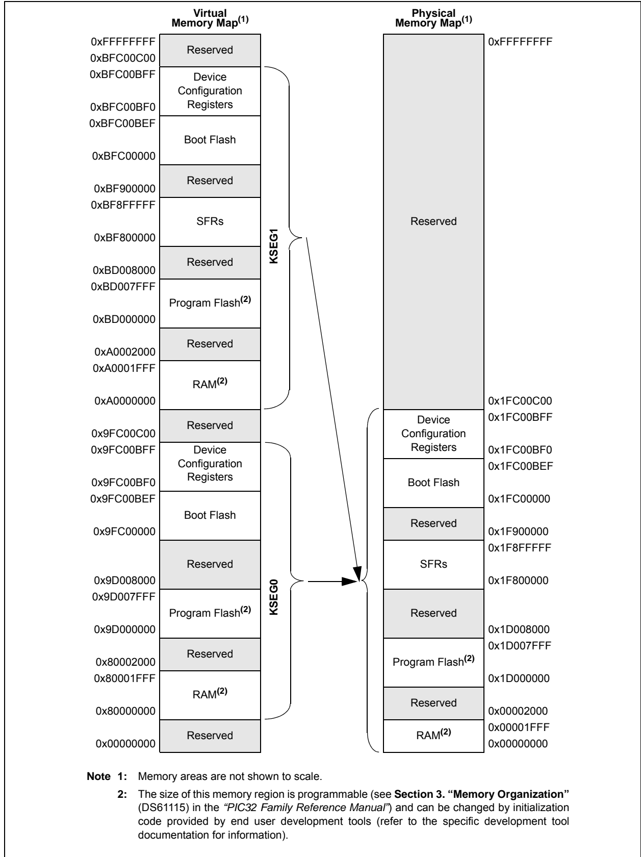
FIGURE 4-2: MEMORY MAP ON RESET FOR PIC32MX12X/22X DEVICES
