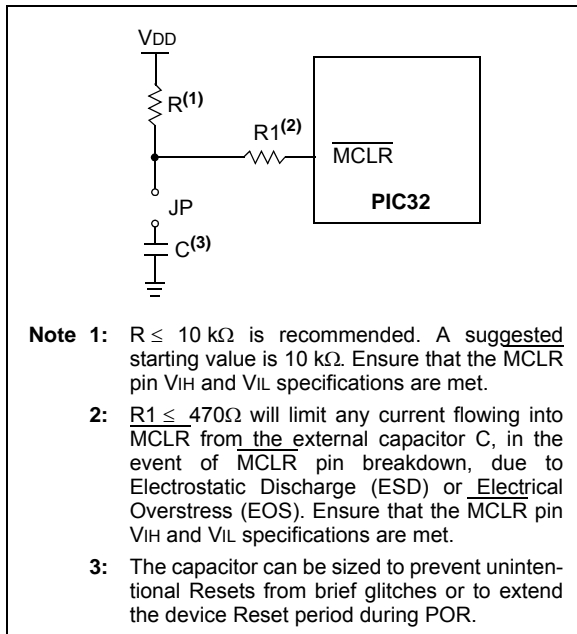
FIGURE 2-2: MCLR PIN CONNECTIONS
