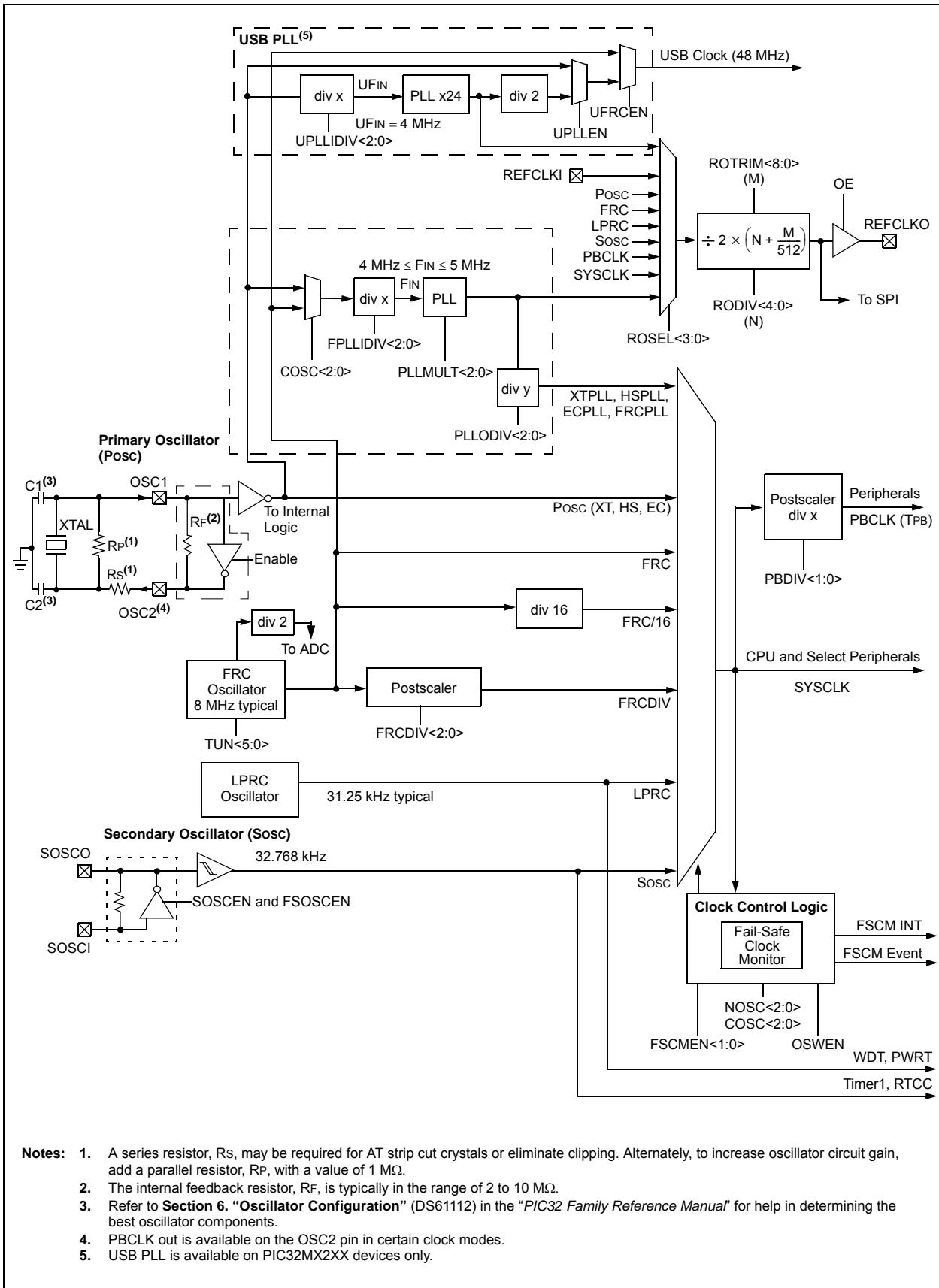
FIGURE 8-1: OSCILLATOR DIAGRAM
