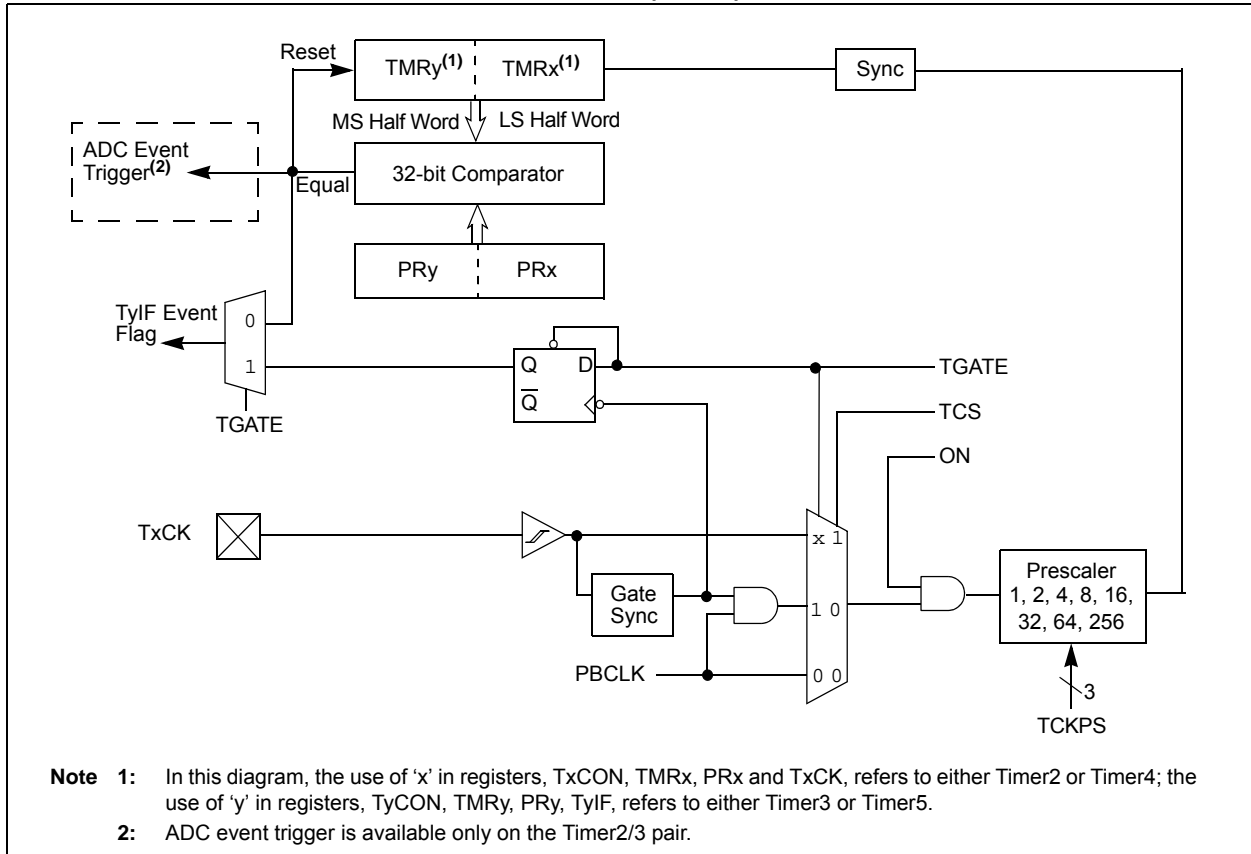
FIGURE 13-2: TIMER2/3, 4/5 BLOCK DIAGRAM (32-BIT)
