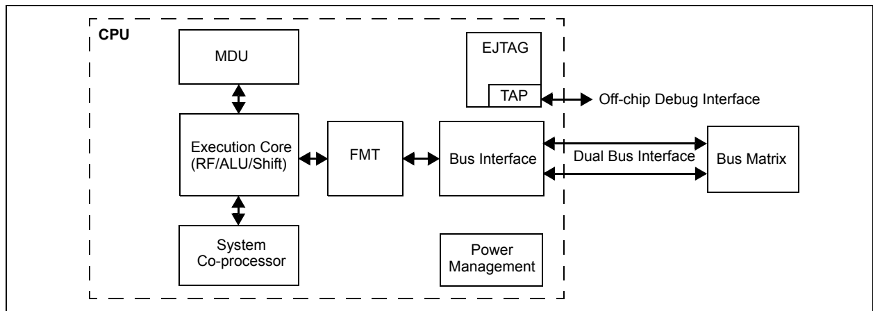
FIGURE 3-1: MIPS32® M4K® PROCESSOR CORE BLOCK DIAGRAM
