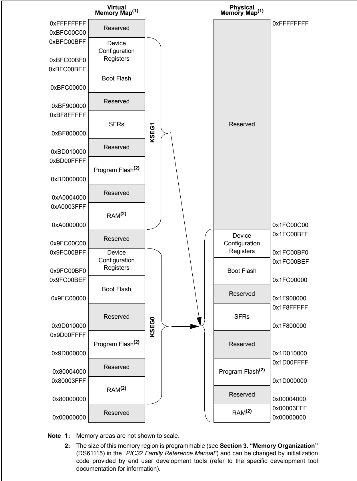
FIGURE 4-3: MEMORY MAP ON RESET FOR PIC32MX13X/23X DEVICES
