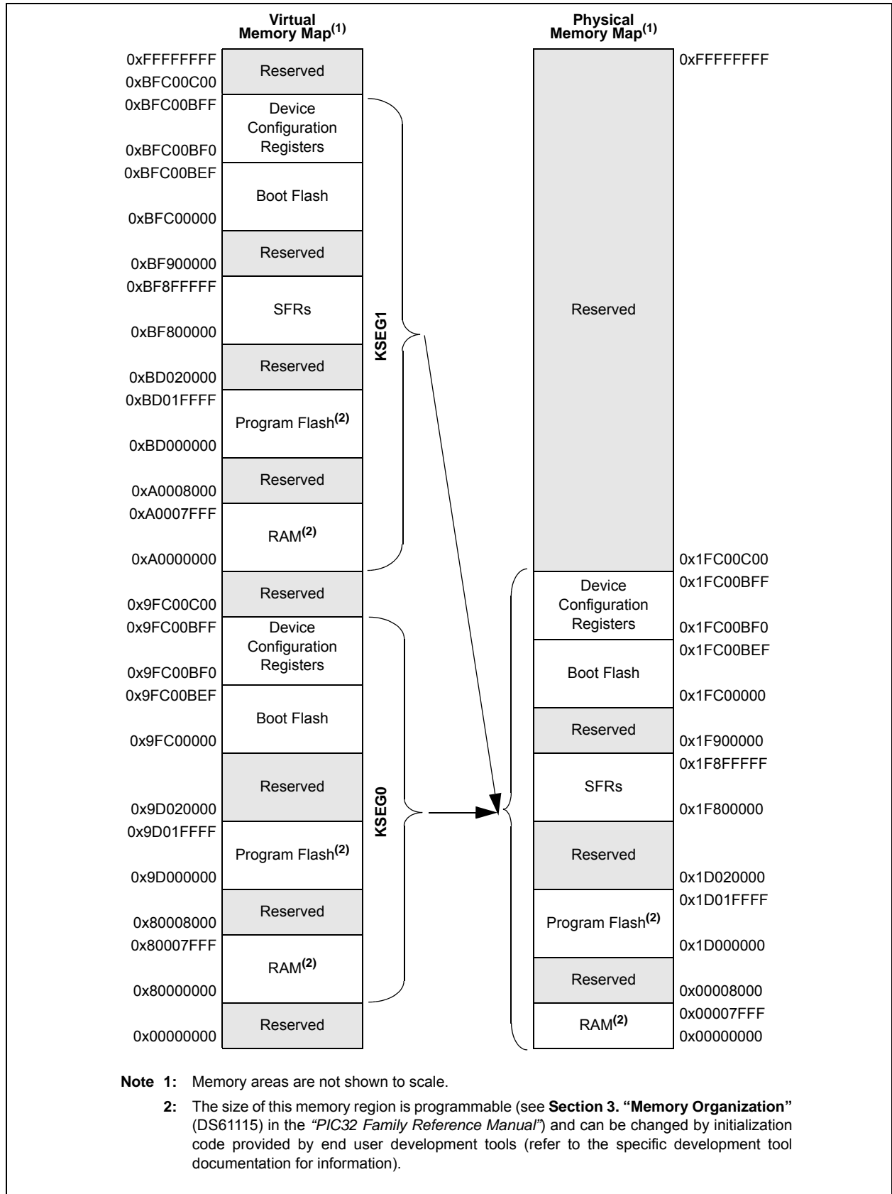
FIGURE 4-4: MEMORY MAP ON RESET FOR PIC32MX15X/25X DEVICES
