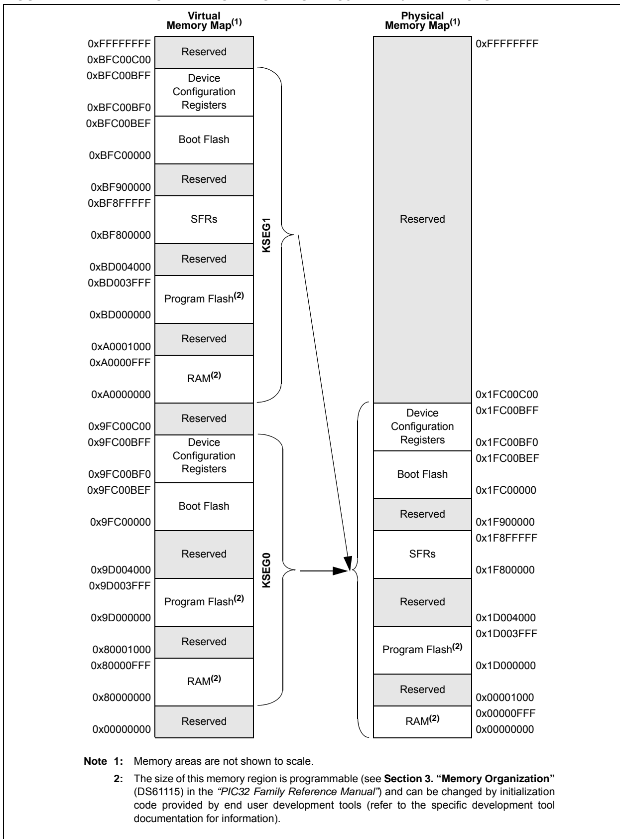
FIGURE 4-1: MEMORY MAP ON RESET FOR PIC32MX11X/21X DEVICES
