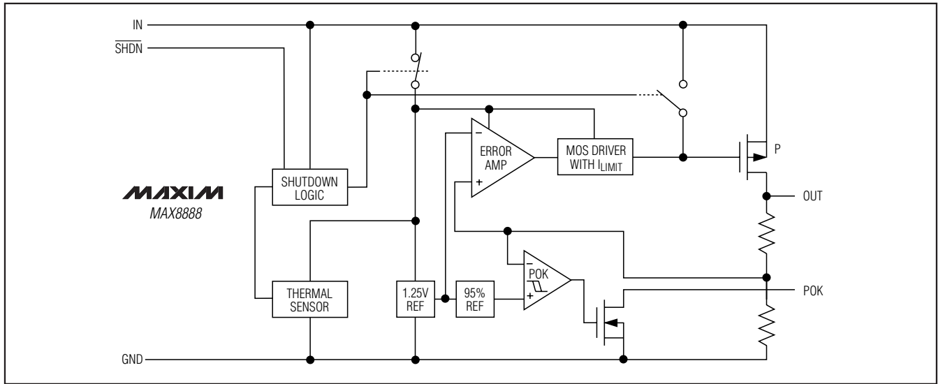
Figure 1. Functional Diagram
