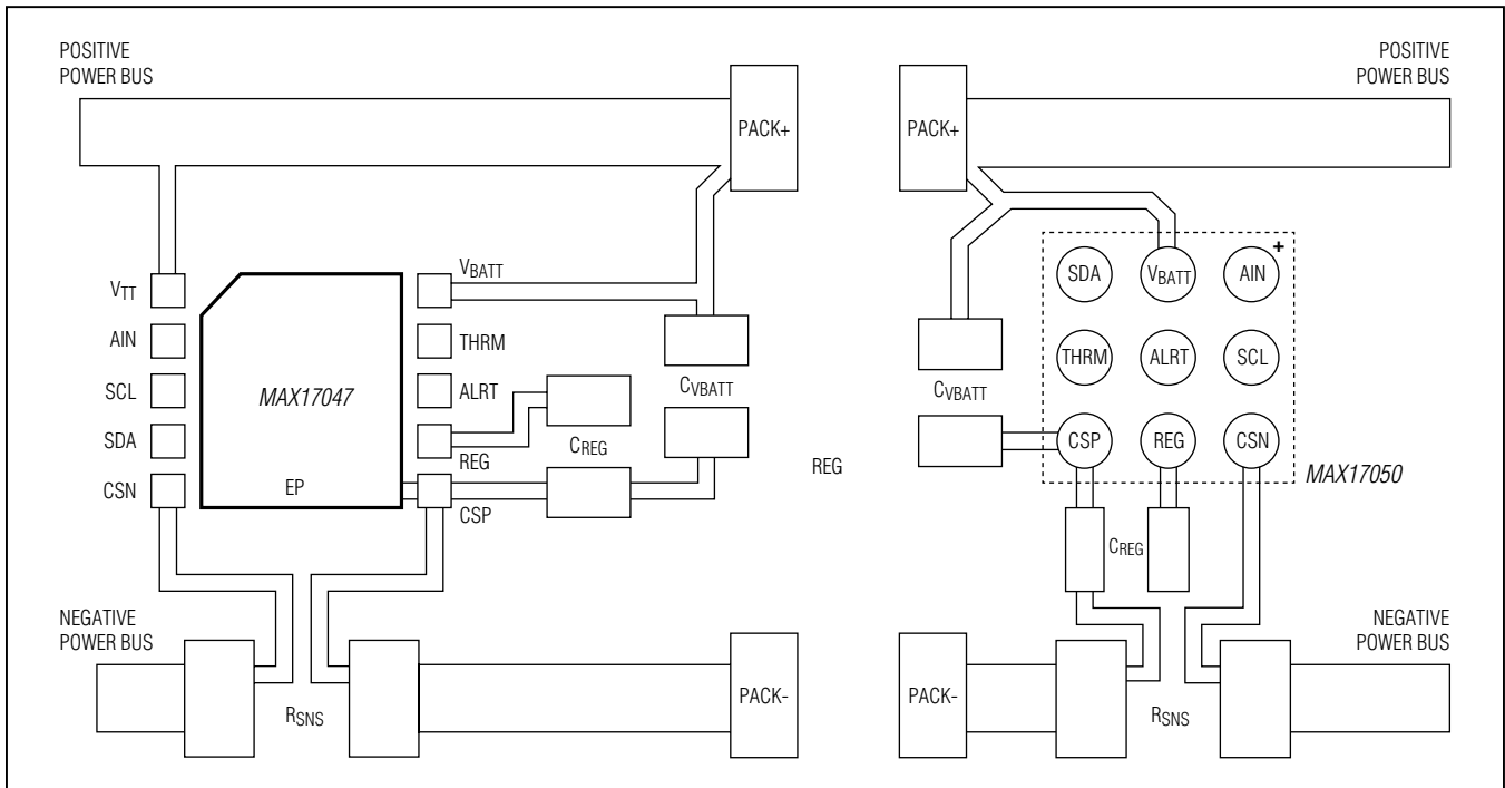
Figure 8. Proper Board Layout
