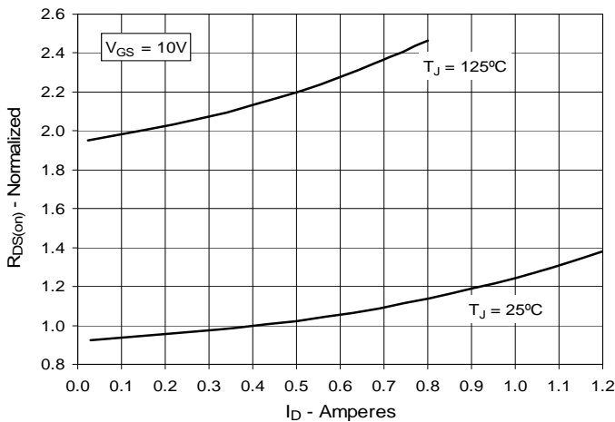
Fig. 5. R_{DS(on)} Normalized to I_D = 0.4A Value vs. Drain Current
