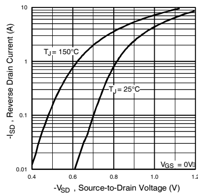
Fig 14. Typical Source-Drain Diode Forward Voltage
