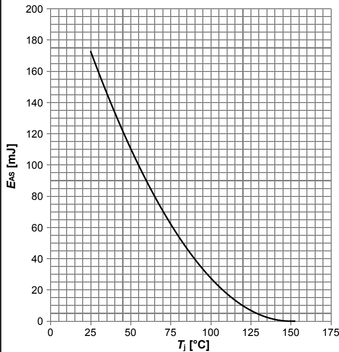
Avalanche energy
