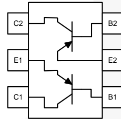
Figure 4. FMB2907A Internal Connections
