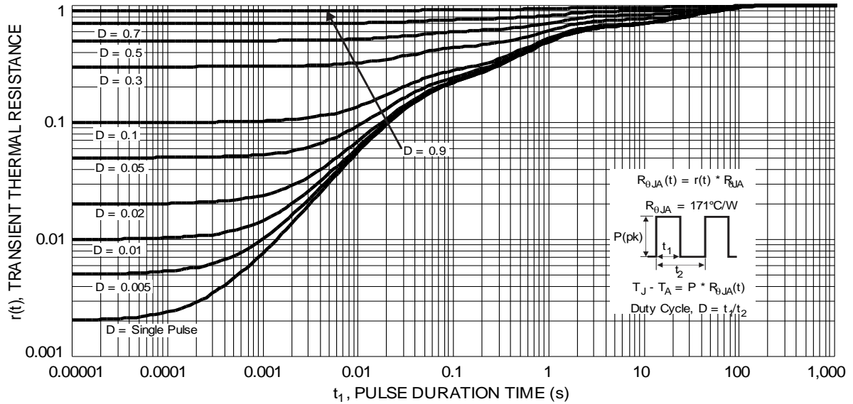
Figure 12 Transient Thermal Response
