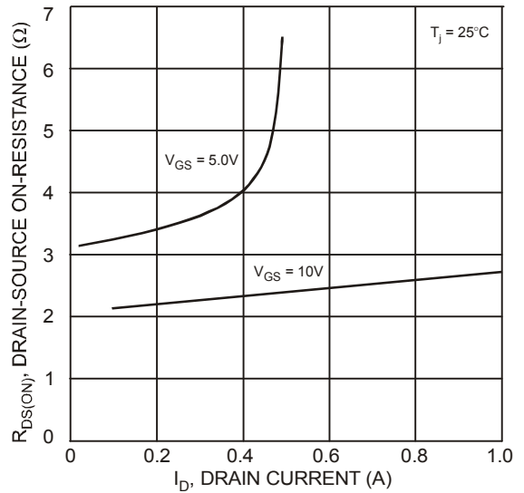
Fig. 9 On-Resistance vs. Drain Current (2N7002)
