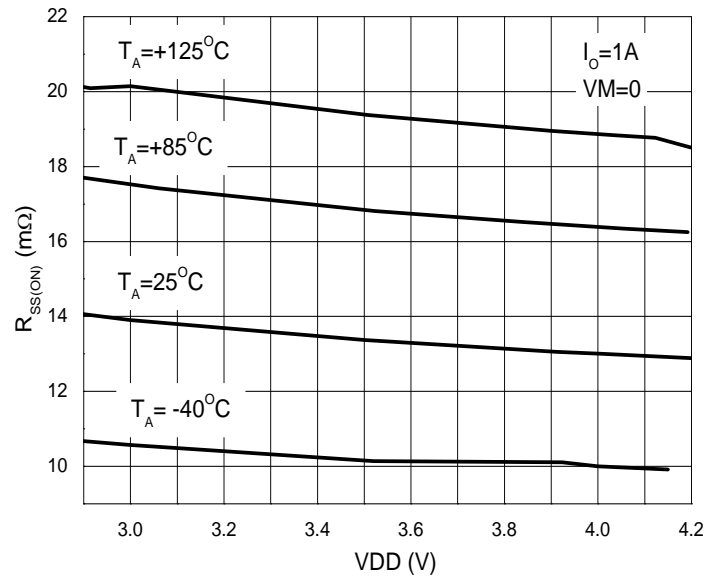
R_{SS(ON)} Characteristics
