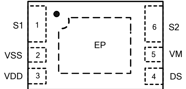
U-DFN2535-6
