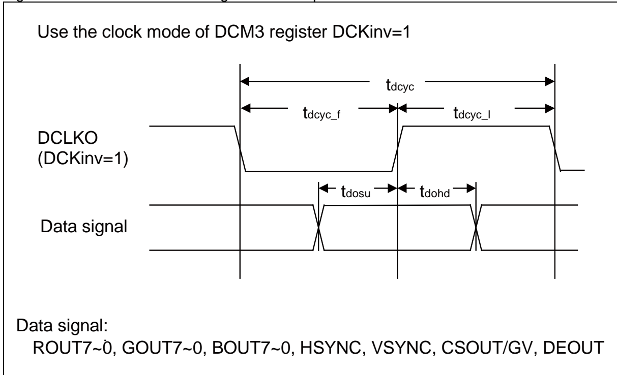
Figure 2 Built-in PLL Reverse Edge Mode Setup/Hold Definition
