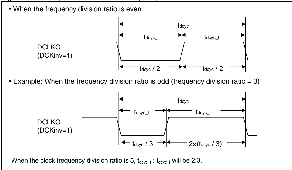
Figure 1 Clock duty ratio when the clock frequency division ratio is even or odd
