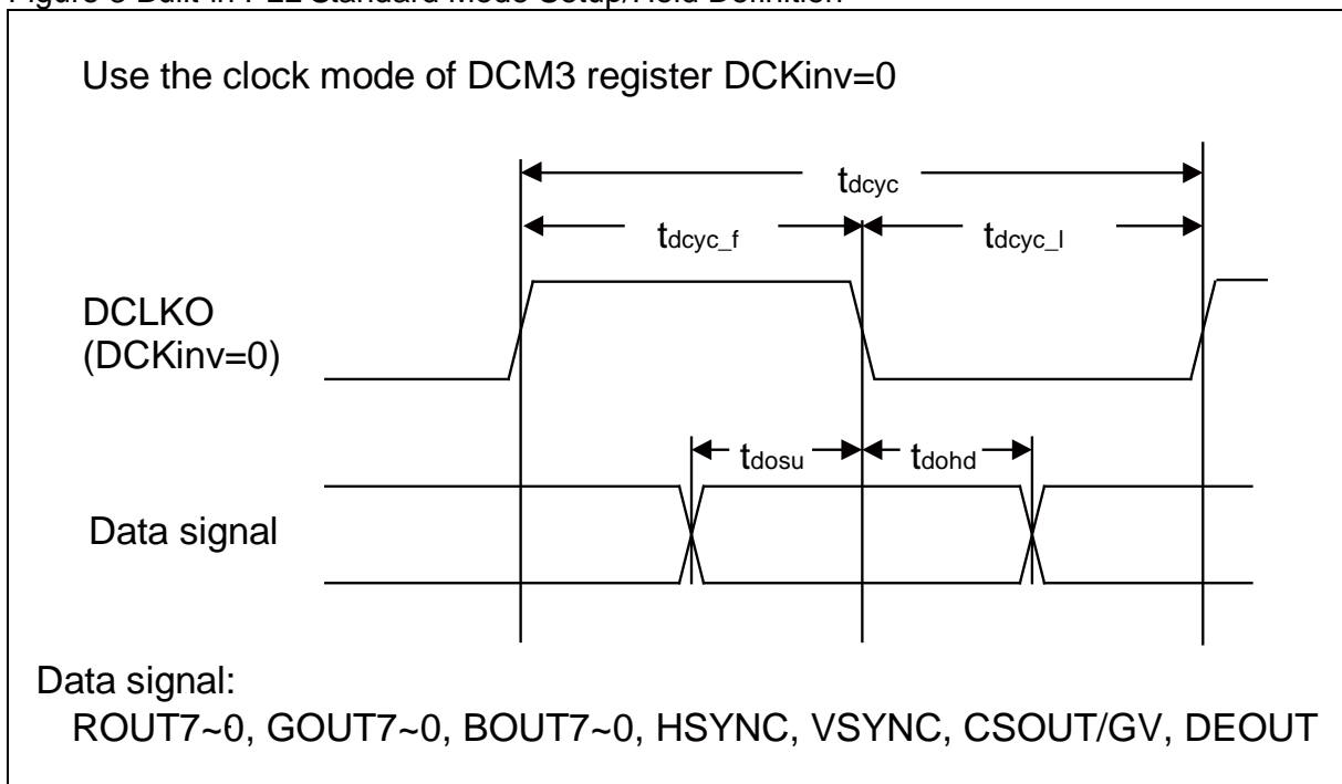
Figure 3 Built-in PLL Standard Mode Setup/Hold Definition
