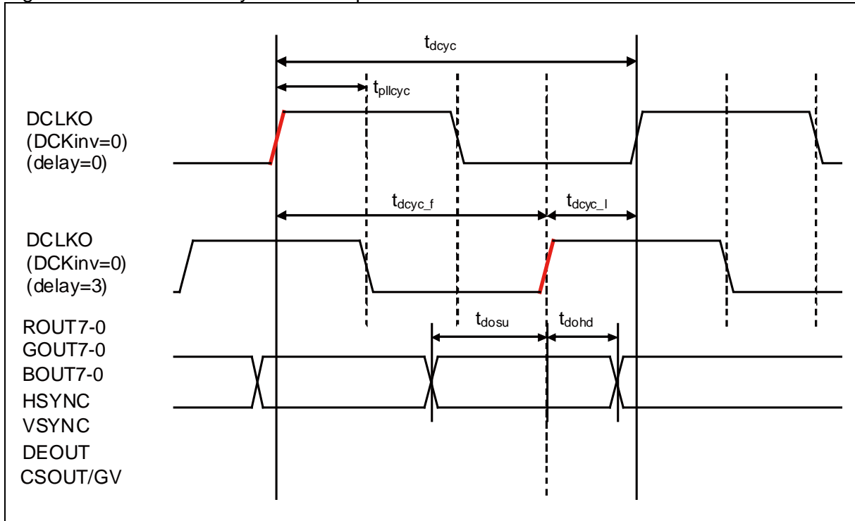
Figure 4 Built-in PLL Delay Mode Setup/Hold Definition
