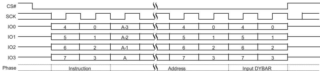
Figure 9.58 DYBWR QPI Mode Command Sequence
