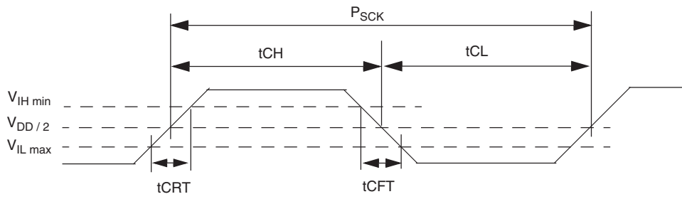
Figure 5.9 Clock Timing
