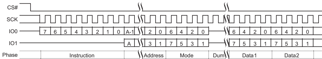
Figure 9.30 Dual I/O Read Command Sequence (BBh)
