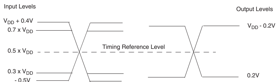
Figure 5.3 Input, Output, and Timing Reference Levels
