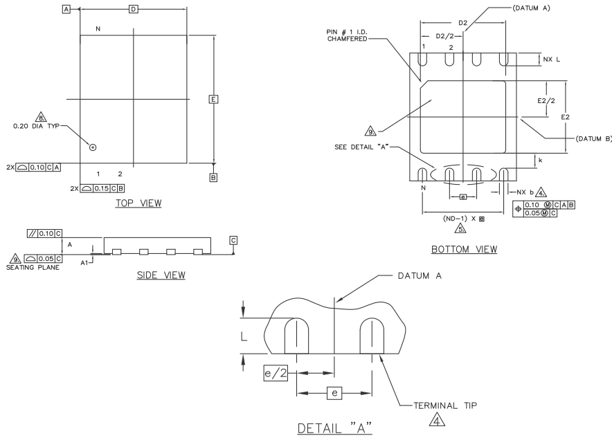
Figure 6.6 WSON 8-Contact 6x5 mm Leadless (WND008)
