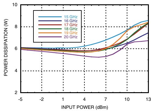
Power Dissipation
