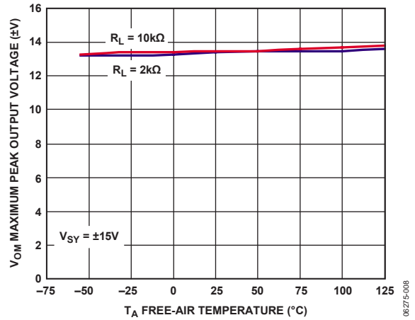
Figure 8. Maximum Peak Output Voltage vs. Free-Air Temperature
