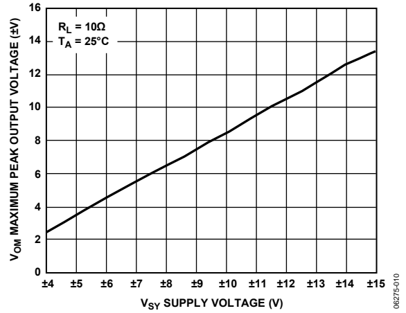
Figure 10. Maximum Peak Output Voltage vs. Supply Voltage
