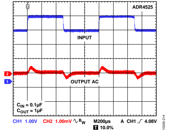
Figure 29. ADR4525 Line Transient Response
