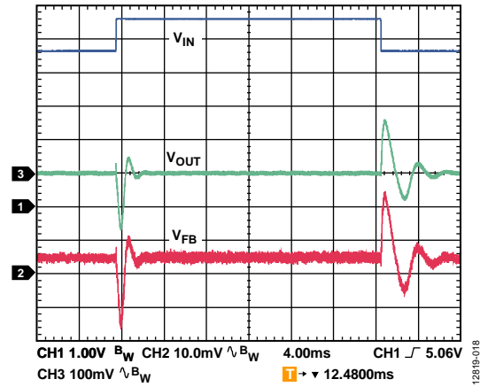
Figure 18. Line Transient Showing V_{IN} , V_{OUT} , and V_{FB} , V_{IN} = 4.5\text{ V} to 5.5\text{ V} Step, V_{NEG} = -12\text{ V} , R_{LOAD} = 300\ \Omega , f_{SW} = 1.2\text{ MHz} , T_A = 25^\circ\text{C}
