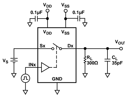
Figure 17. Switching Times
