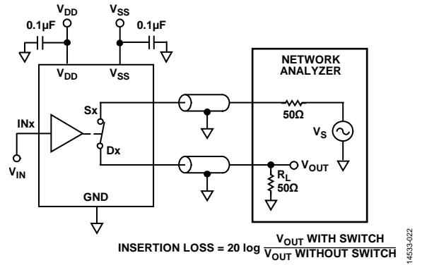
Figure 22. Bandwidth
