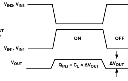
Figure 19. Charge Injection
