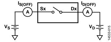
Figure 15. Off Leakage
