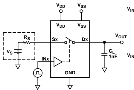
Figure 19. Charge Injection
