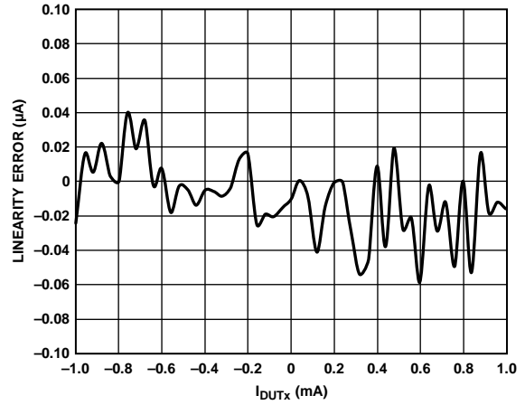
Figure 108. PPMU Measure Current INL, Range B
