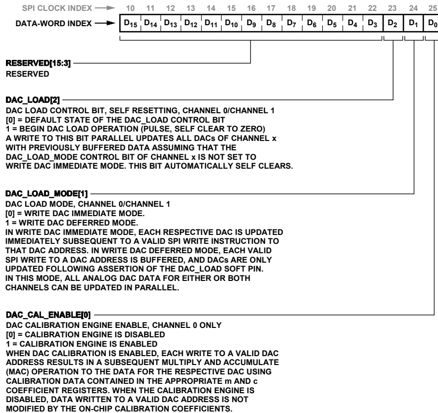
Figure 146. DAC Control Register (Address 0x11)
