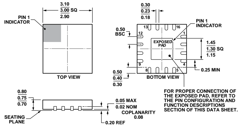
Figure 68. 16-Lead Lead Frame Chip Scale Package [LFCS] 3 mm × 3 mm Body and 0.75 mm Package Height (CP-16-21) Dimensions shown in millimeters
