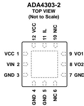
Figure 4. Pin Configuration
