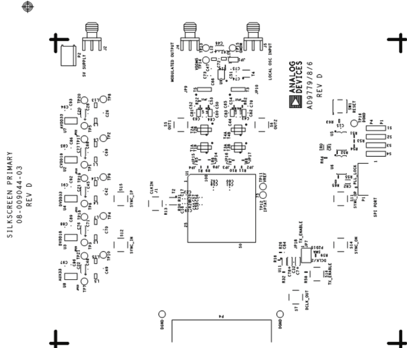
Figure 110. Evaluation Board, Rev. D, Top Silk Screen
