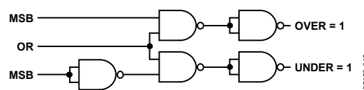
Figure 56. Overrange/Underrange Logic
