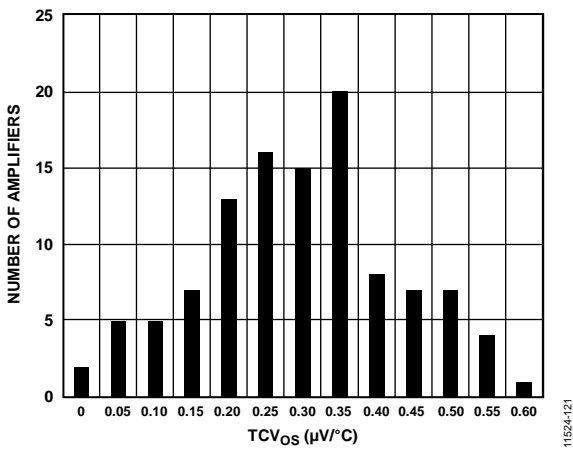
Figure 4. TCV_{OS} Distribution, SOIC Package, V_{SY} = \pm 15.0\text{ V}
