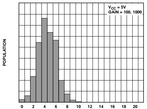
Figure 10. Input Offset Voltage (µV)
