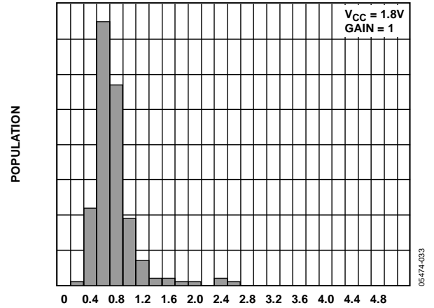
Figure 28. Input Offset Voltage Drift ( \mu V/^{\circ}C )
