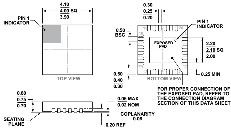
Figure 41. 24-Lead Lead Frame Chip Scale Package [LFCSQ] 4 mm × 4 mm Body, Very Very Thin Quad (CP-24-10) Dimensions shown in millimeters
