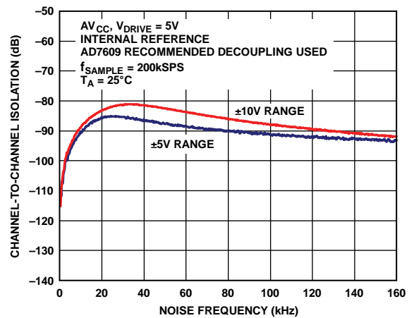
Figure 25. Channel-to-Channel Isolation
