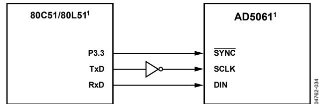
Figure 43. AD5061-to-80C51/80L51 Interface
