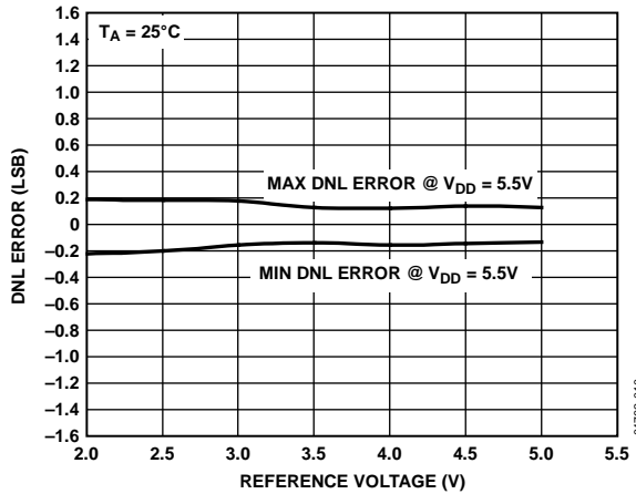
Figure 10. DNL vs. Reference Input Voltage
