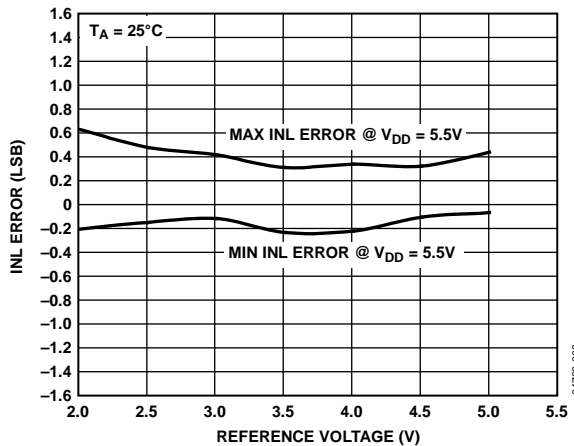
Figure 12. INL vs. Reference Input Voltage
