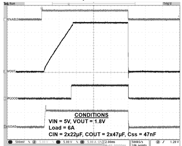
Startup Waveform
