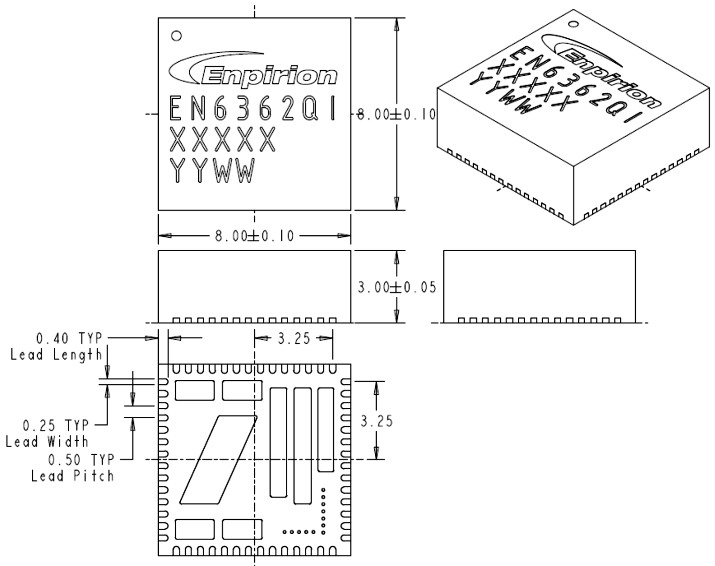
Figure 12: EN6362QI Package Dimensions
