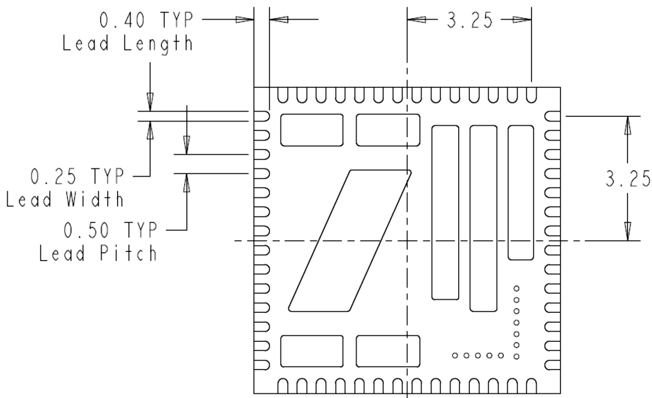
Figure 9: Lead-Frame exposed metal (Bottom View)
