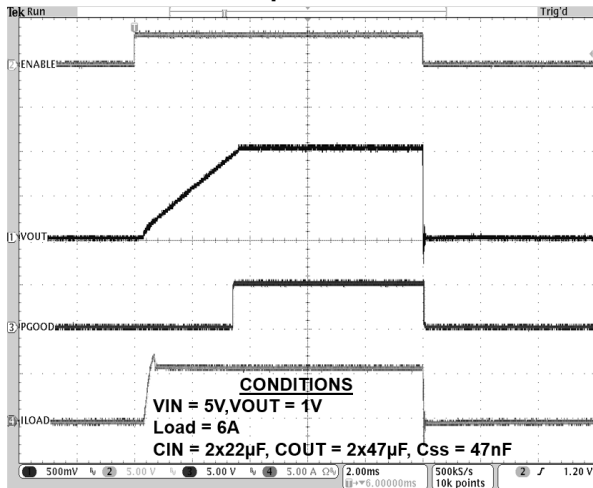
Startup Waveform
