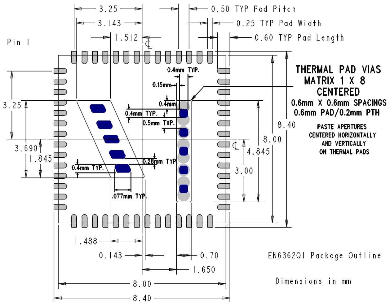
Figure 11: Solder stencil drawing (Top View)
