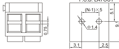
Pitch:5mm
