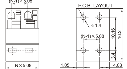
Pitch:5.08mm
