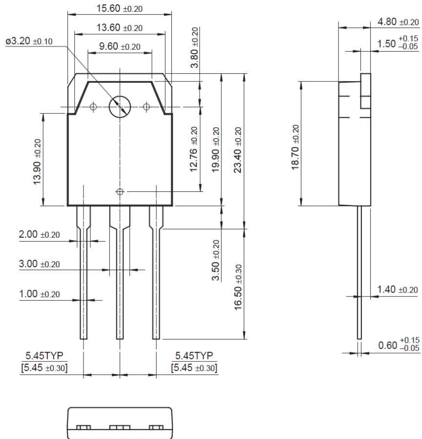
Fig8. Package Outline
