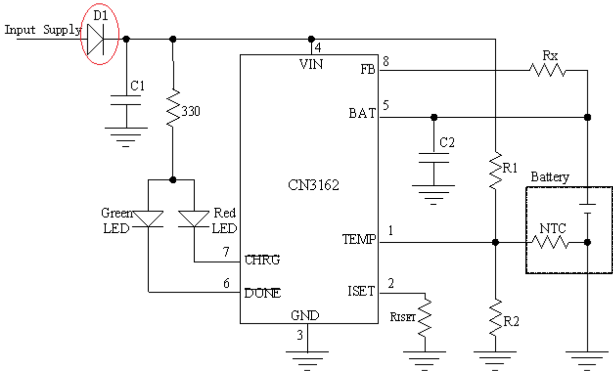
Figure 6 Adding Diode D1 to Suppress Voltage Spike
