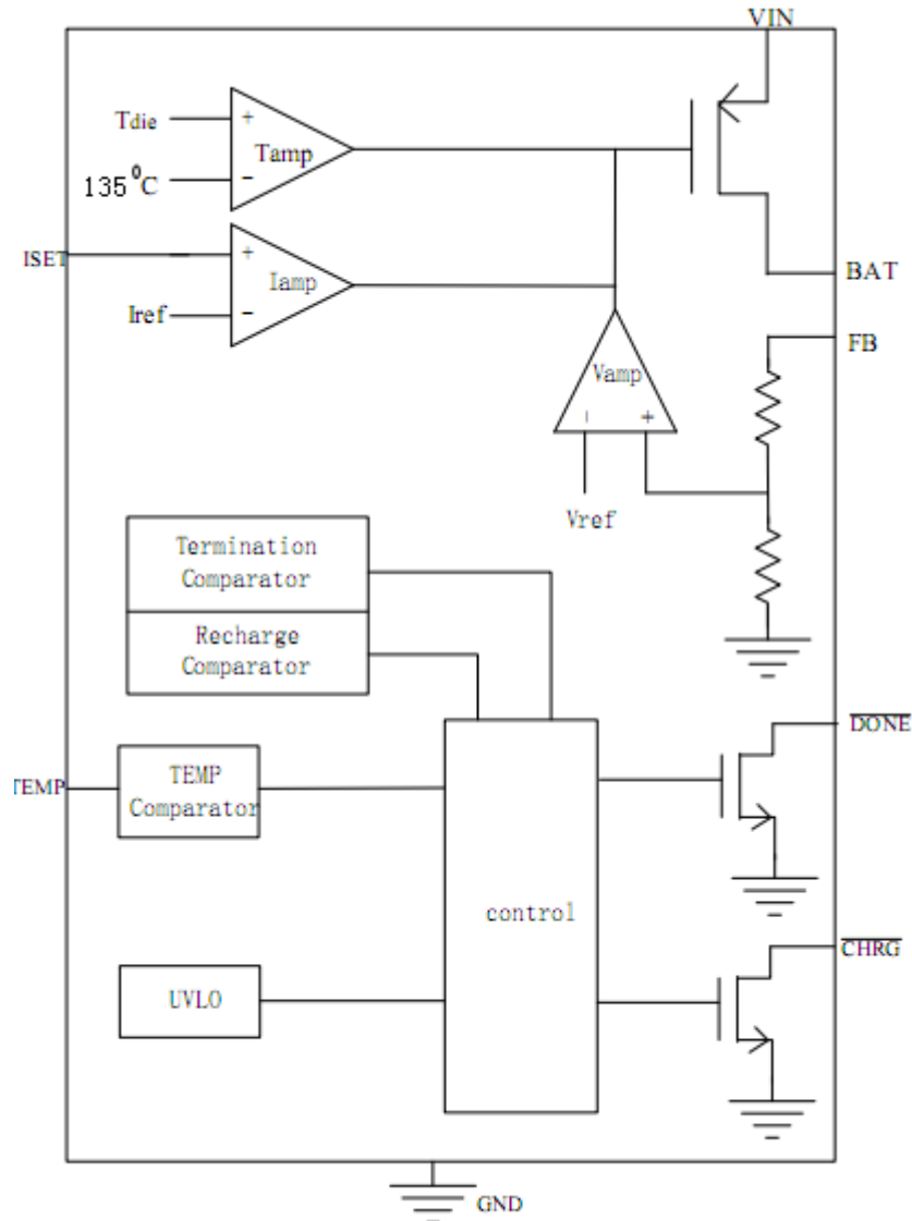
Figure 3 Block Diagram
